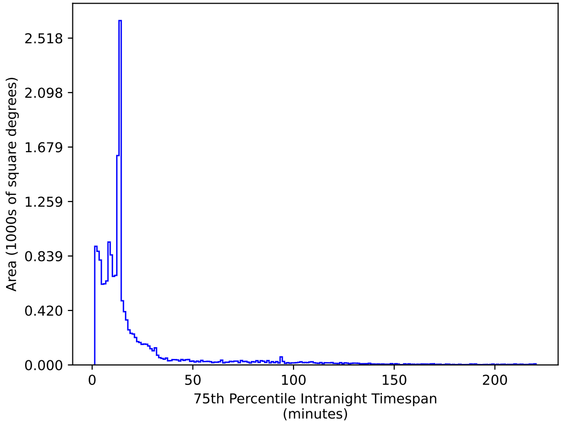
ddf_loaded_half_fl15_v3.4_10yrs WFD z band: 75th Percentile Intranight Timespan
