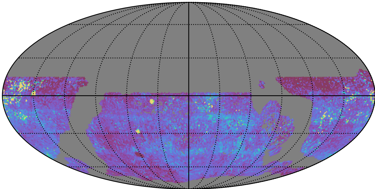
ddf_loaded_half_fl15_v3.4_10yrs WFD y band: 75th Percentile Intranight Timespan
