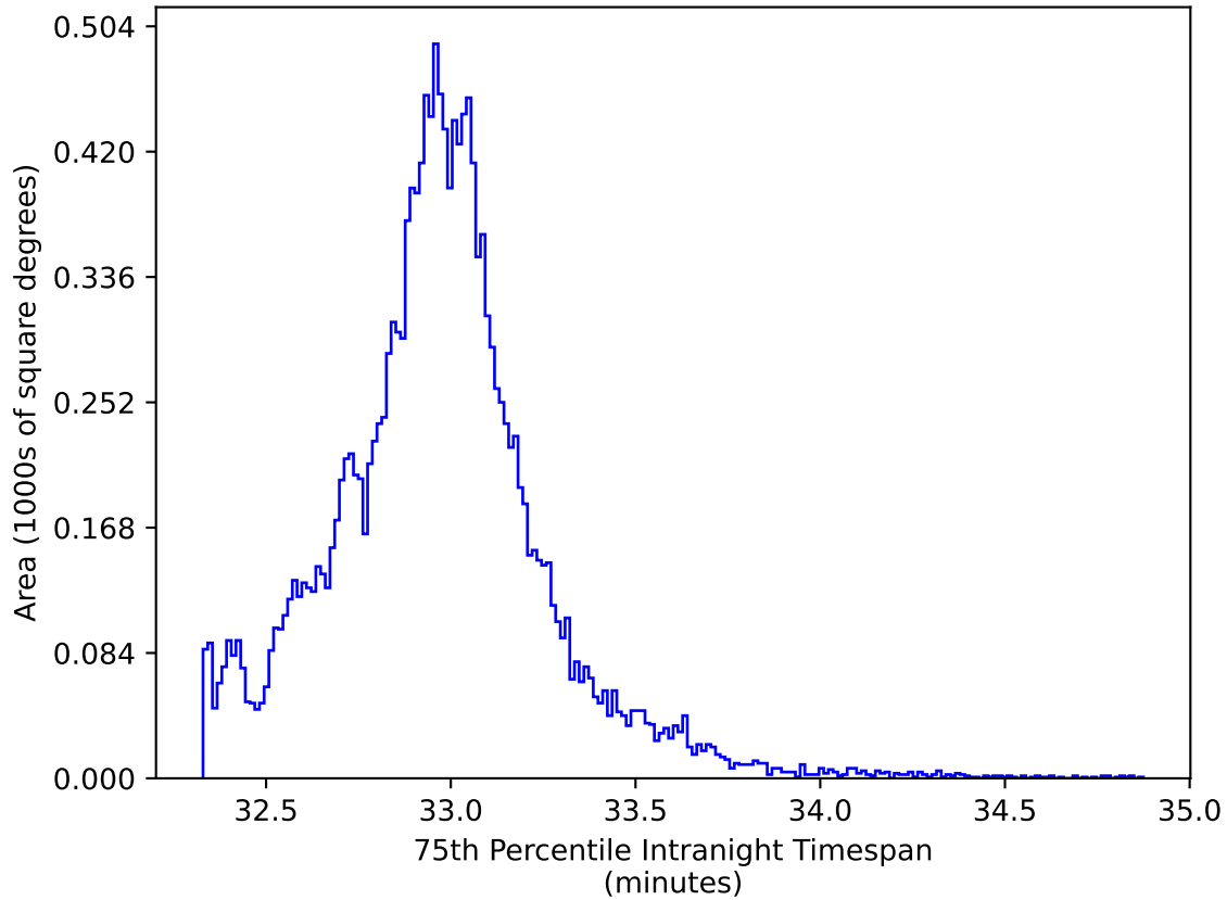
ddf_loaded_half_fl15_v3.4_10yrs WFD y band: 75th Percentile Intranight Timespan
