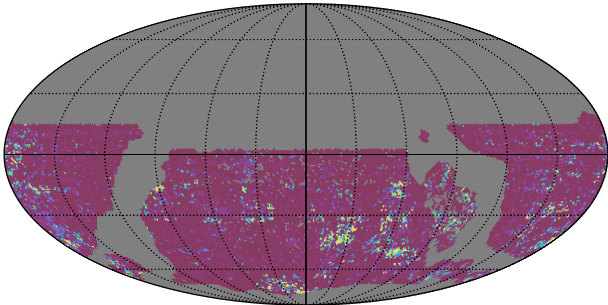
ddf_loaded_half_fl15_v3.4_10yrs WFD u band: 75th Percentile Intranight Timespan
