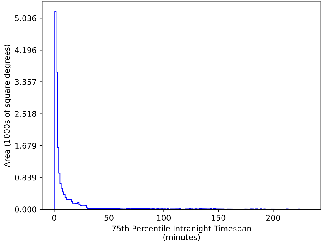
ddf_loaded_half_fl15_v3.4_10yrs WFD u band: 75th Percentile Intranight Timespan
