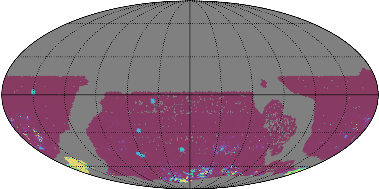
ddf_loaded_half_fl15_v3.4_10yrs WFD ri bands: 75th Percentile Intranight Timespan
