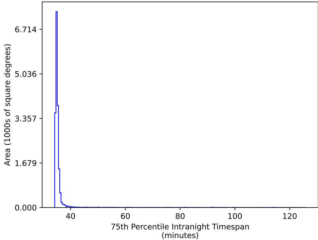
ddf_loaded_half_fl15_v3.4_10yrs WFD ri bands: 75th Percentile Intranight Timespan
