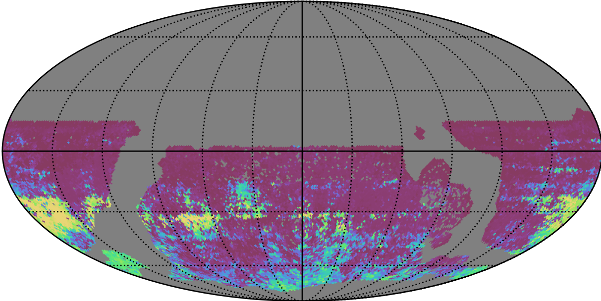
ddf_loaded_half_fl15_v3.4_10yrs WFD r band: 75th Percentile Intranight Timespan
