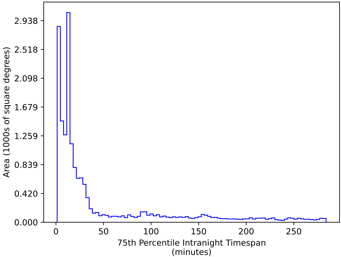
ddf_loaded_half_fl15_v3.4_10yrs WFD r band: 75th Percentile Intranight Timespan
