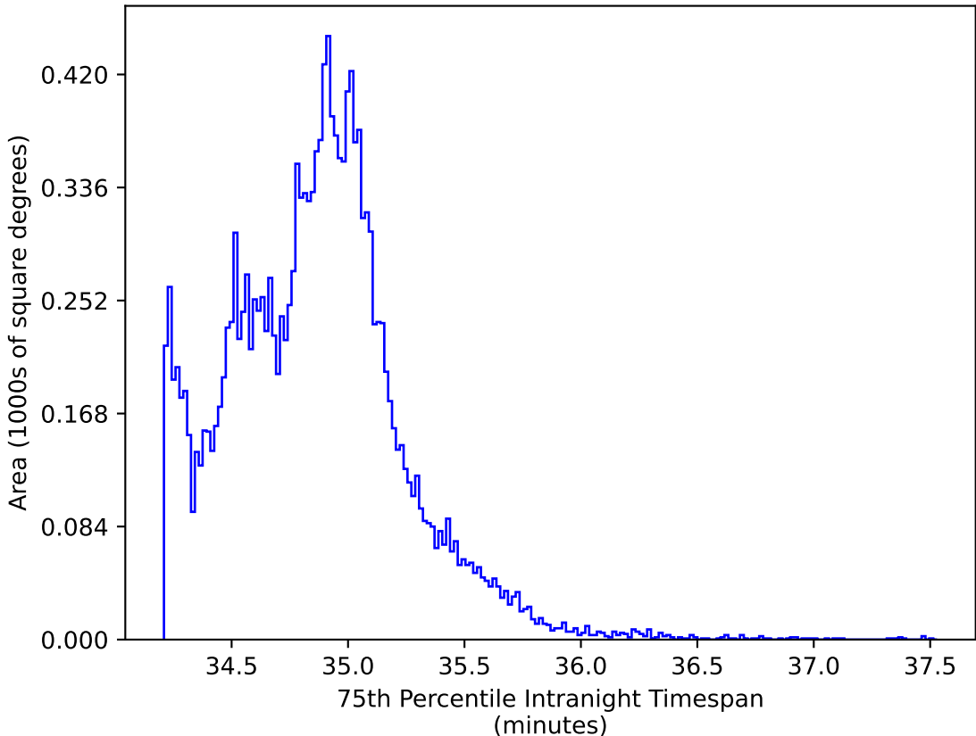
ddf_loaded_half_fl15_v3.4_10yrs WFD iz bands: 75th Percentile Intranight Timespan
