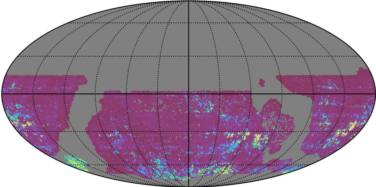
ddf_loaded_half_fl15_v3.4_10yrs WFD i band: 75th Percentile Intranight Timespan
