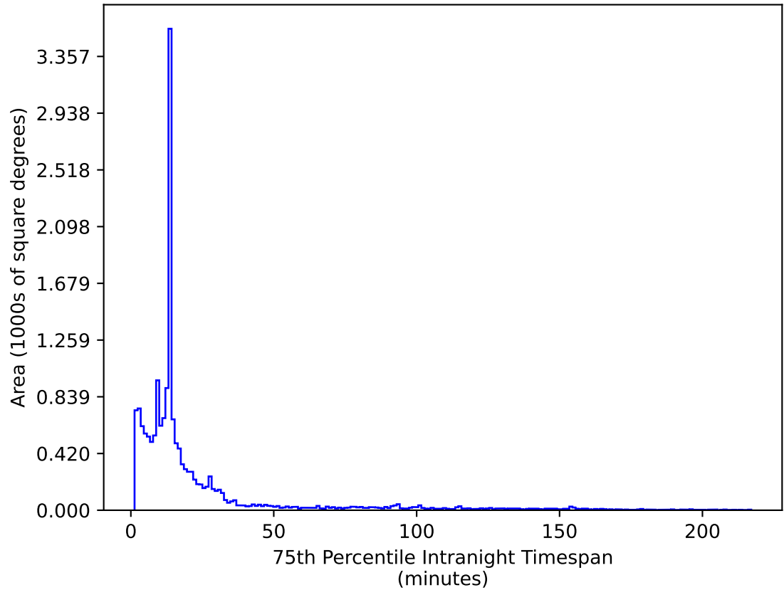
ddf_loaded_half_fl15_v3.4_10yrs WFD i band: 75th Percentile Intranight Timespan
