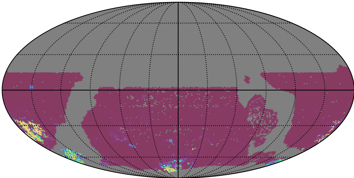
ddf_loaded_half_fl15_v3.4_10yrs WFD gr bands: 75th Percentile Intranight Timespan
