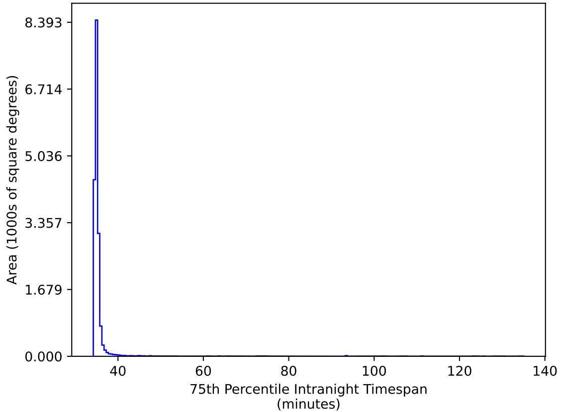
ddf_loaded_half_fl15_v3.4_10yrs WFD gr bands: 75th Percentile Intranight Timespan
