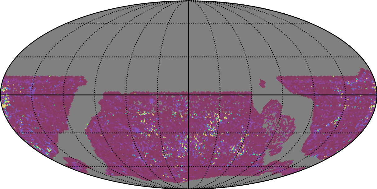
ddf_loaded_half_fl15_v3.4_10yrs WFD g band: 75th Percentile Intranight Timespan
