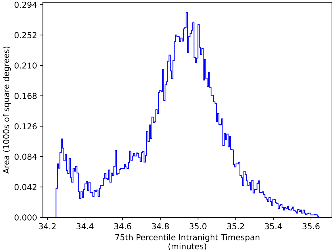
ddf_loaded_half_fl15_v3.4_10yrs WFD all bands: 75th Percentile Intranight Timespan
