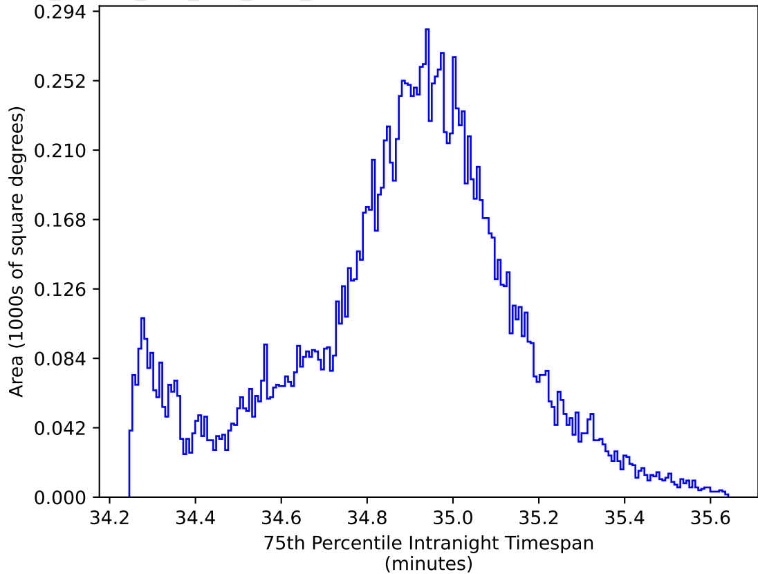
ddf_loaded_half_fl15_v3.4_10yrs WFD: 75th Percentile Intranight Timespan
