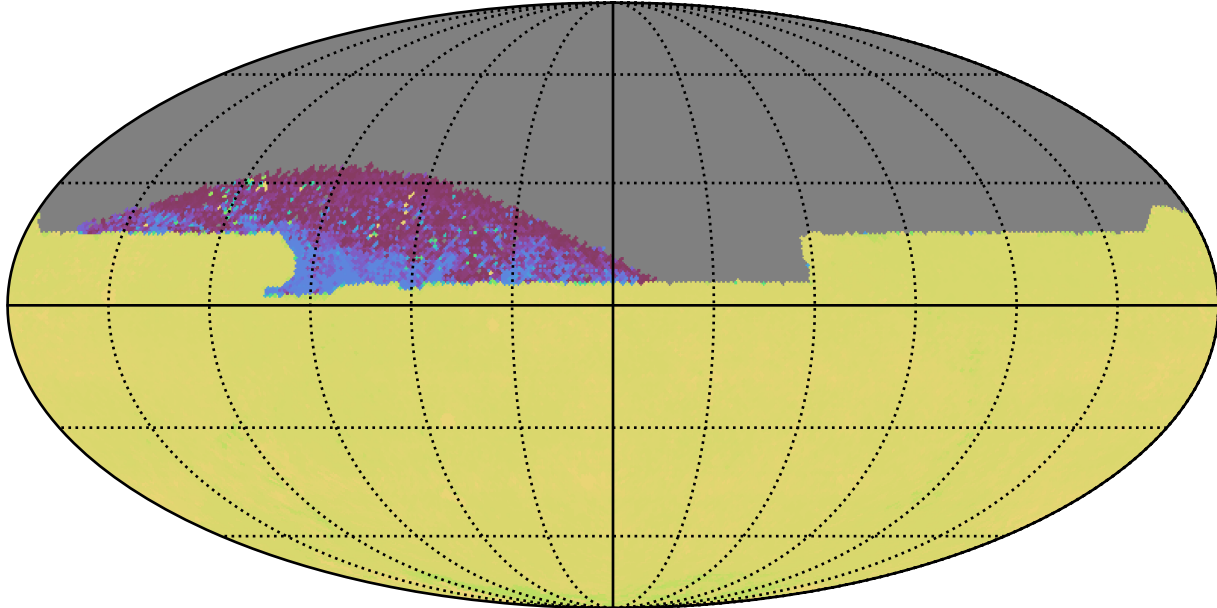
ddf_loaded_half_fl15_v3.4_10yrs All sky zy bands: 75th Percentile Intranight Timespan
