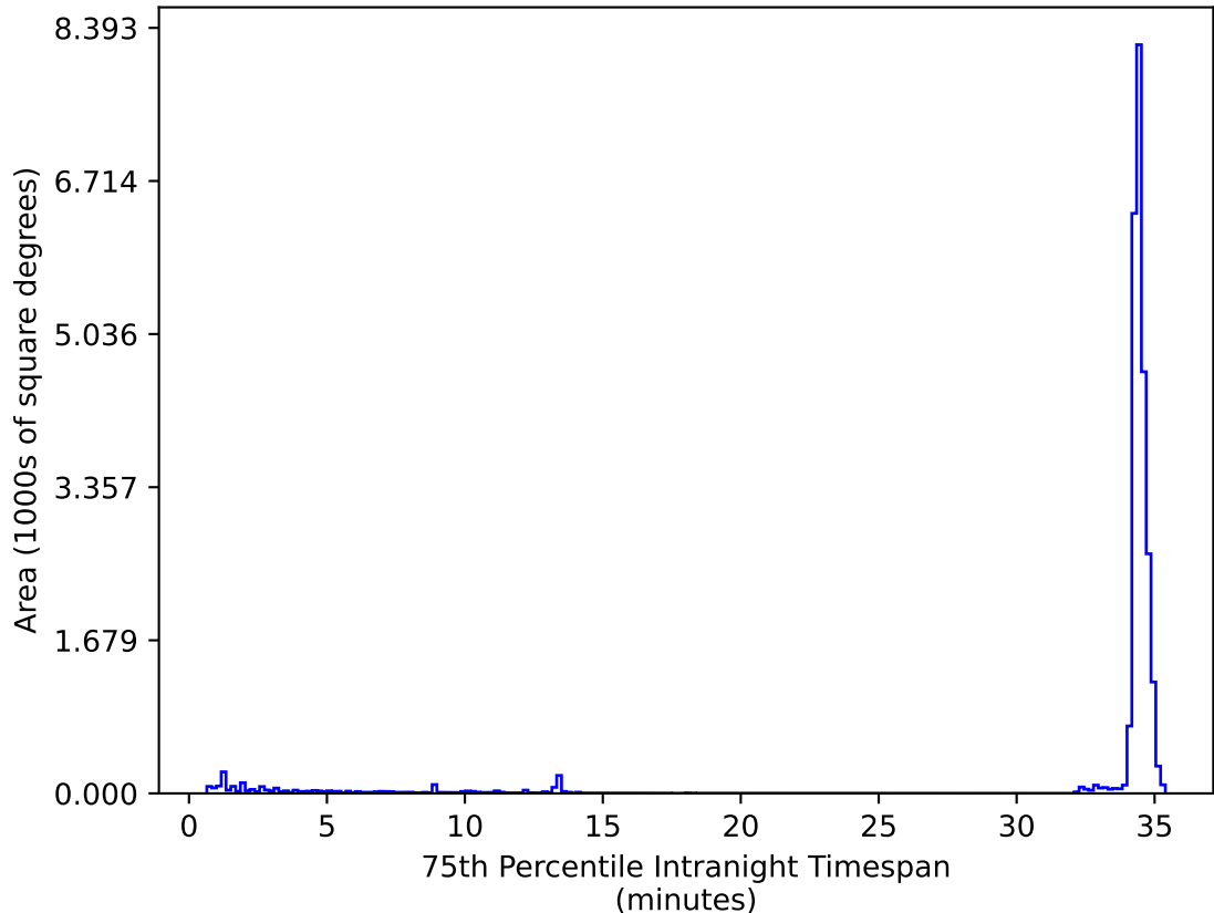
ddf_loaded_half_fl15_v3.4_10yrs All sky zy bands: 75th Percentile Intranight Timespan
