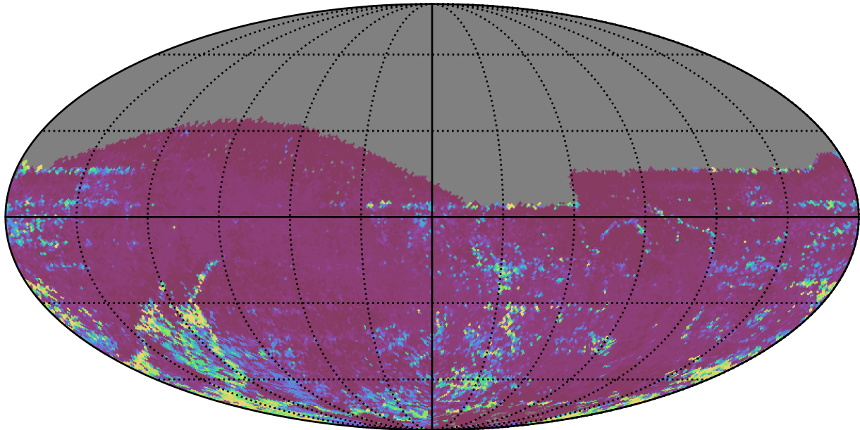
ddf_loaded_half_fl15_v3.4_10yrs All sky z band: 75th Percentile Intranight Timespan
