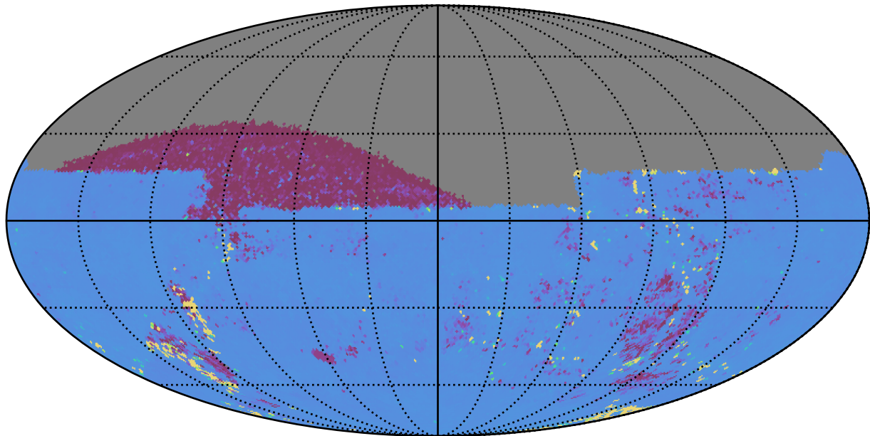
ddf_loaded_half_fl15_v3.4_10yrs All sky ug bands: 75th Percentile Intranight Timespan
