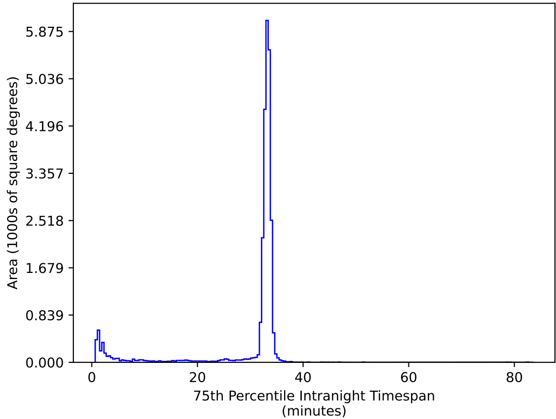
ddf_loaded_half_fl15_v3.4_10yrs All sky ug bands: 75th Percentile Intranight Timespan
