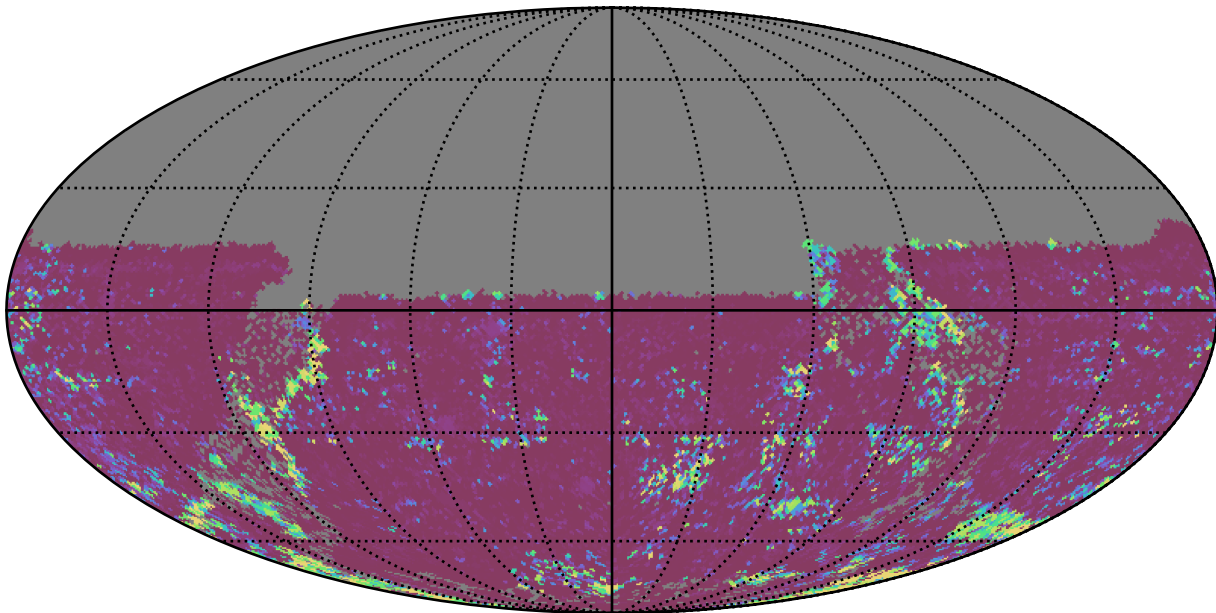
ddf_loaded_half_fl15_v3.4_10yrs All sky u band: 75th Percentile Intranight Timespan
