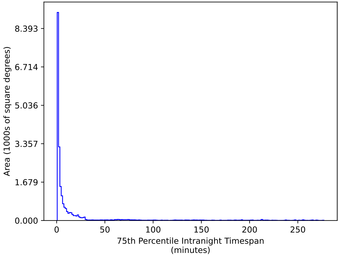
ddf_loaded_half_fl15_v3.4_10yrs All sky u band: 75th Percentile Intranight Timespan
