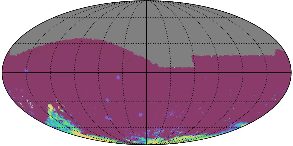
ddf_loaded_half_fl15_v3.4_10yrs All sky ri bands: 75th Percentile Intranight Timespan
