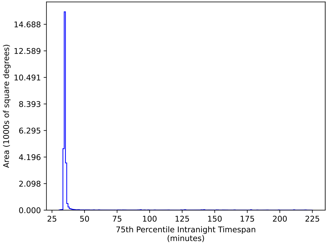
ddf_loaded_half_fl15_v3.4_10yrs All sky ri bands: 75th Percentile Intranight Timespan
