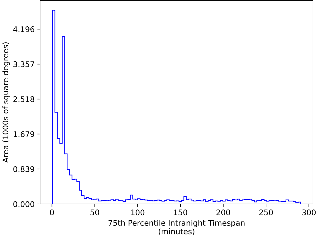
ddf_loaded_half_fl15_v3.4_10yrs All sky r band: 75th Percentile Intranight Timespan
