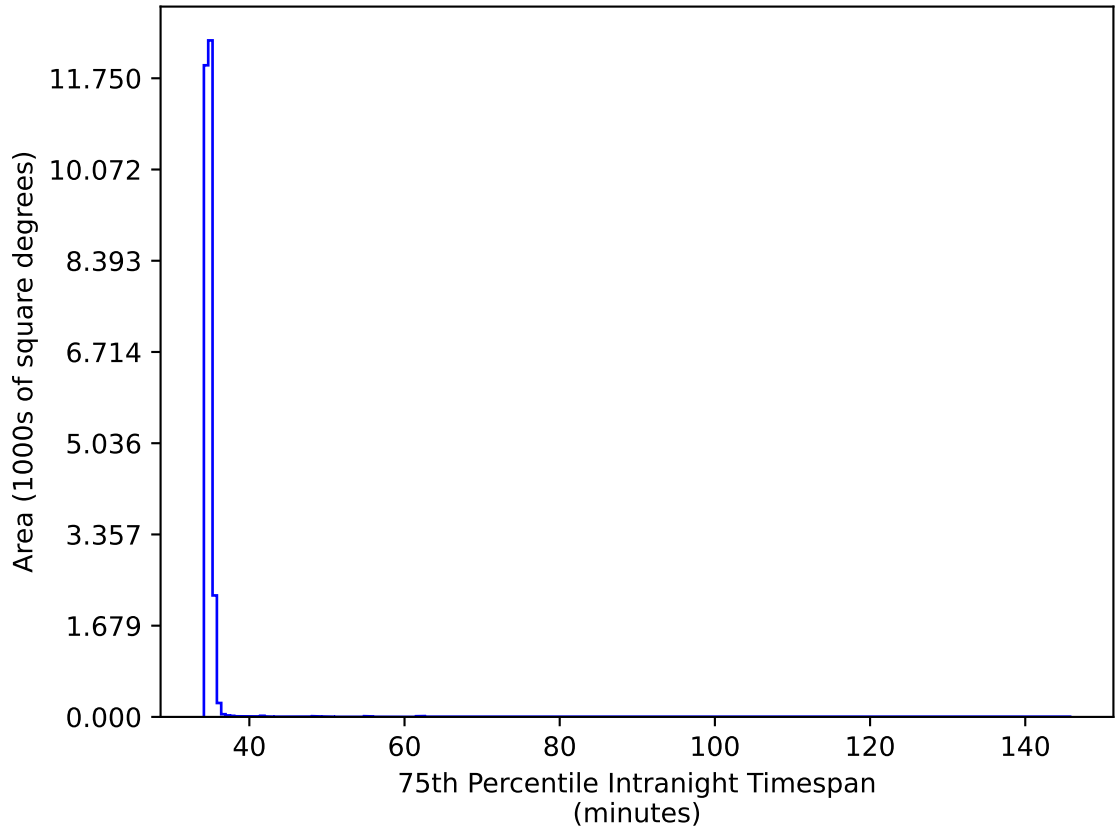
ddf_loaded_half_fl15_v3.4_10yrs All sky iz bands: 75th Percentile Intranight Timespan
