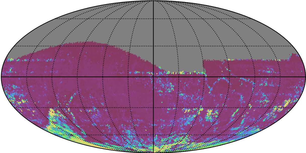
ddf_loaded_half_fl15_v3.4_10yrs All sky i band: 75th Percentile Intranight Timespan
