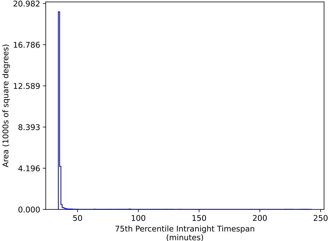
ddf_loaded_half_fl15_v3.4_10yrs All sky gr bands: 75th Percentile Intranight Timespan
