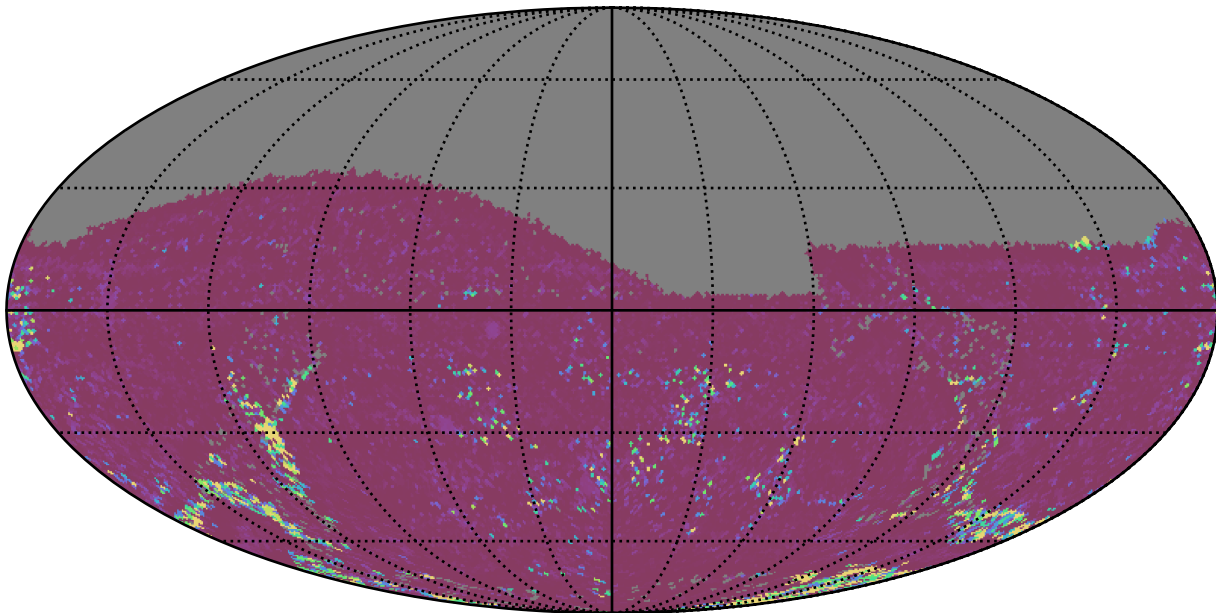
ddf_loaded_half_fl15_v3.4_10yrs All sky g band: 75th Percentile Intranight Timespan
