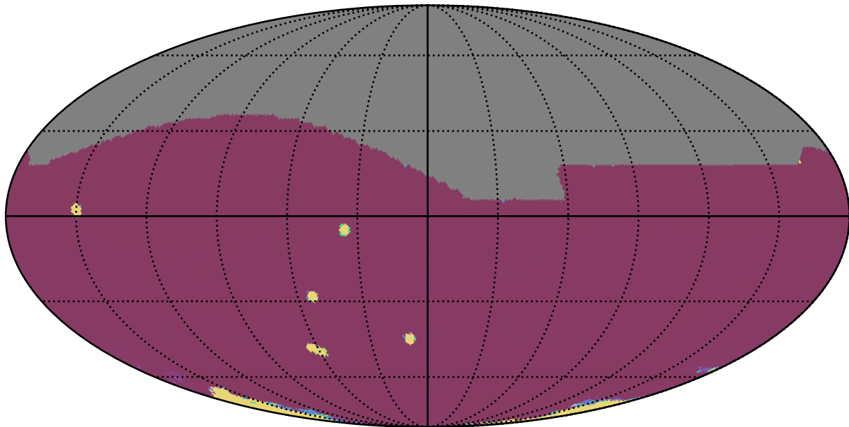
ddf_loaded_half_fl15_v3.4_10yrs All sky all bands: 75th Percentile Intranight Timespan
