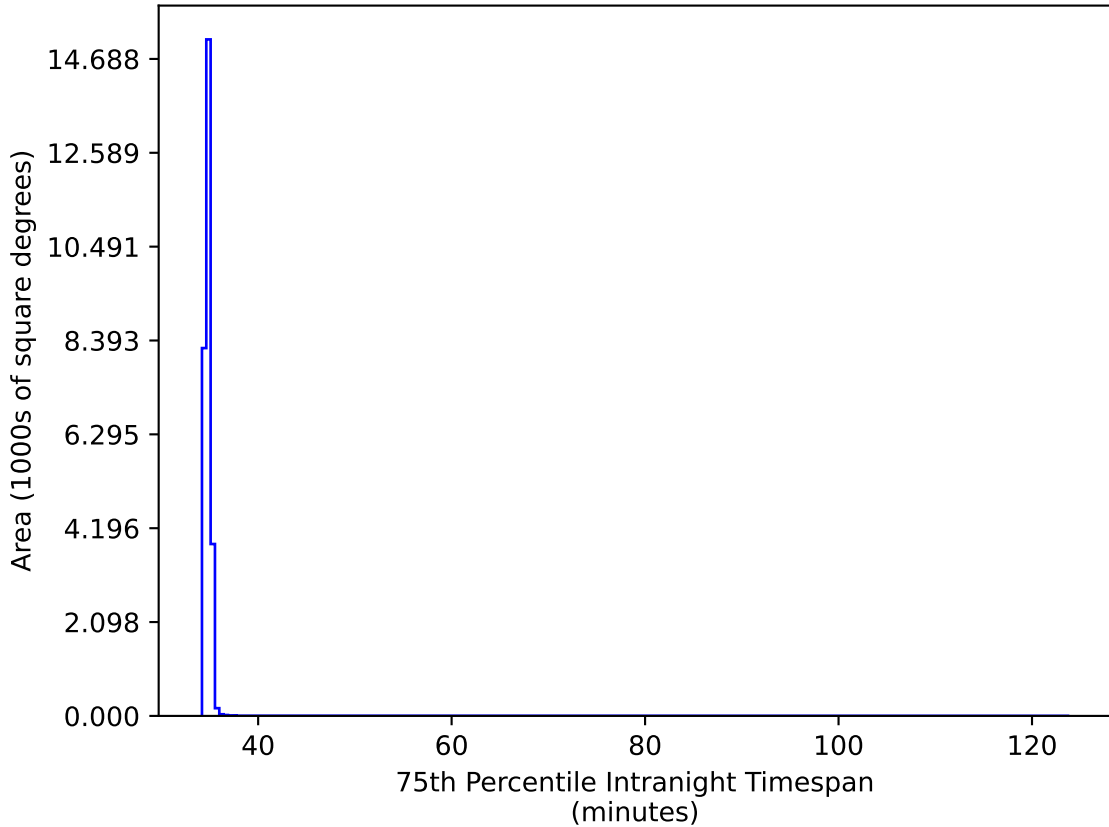
ddf_loaded_half_fl15_v3.4_10yrs All sky: 75th Percentile Intranight Timespan
