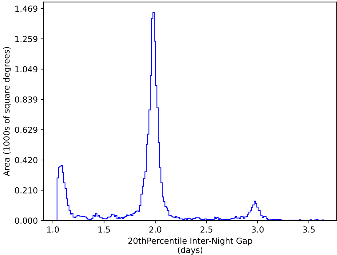
ddf_loaded_half_fl15_v3.4_10yrs WFD y band: 20thPercentile Inter-Night Gap
