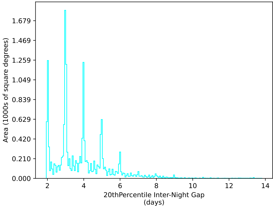
ddf_loaded_half_fl15_v3.4_10yrs WFD u band: 20thPercentile Inter-Night Gap
