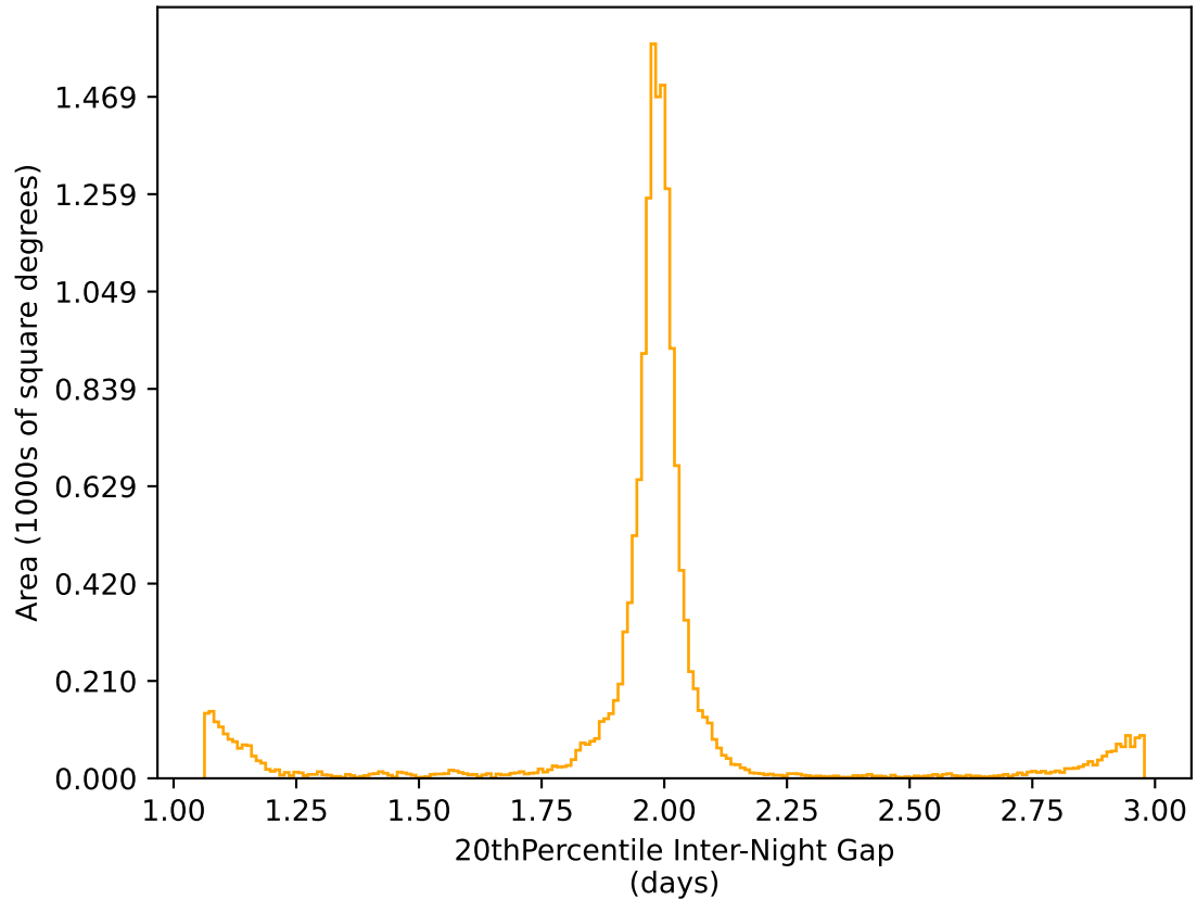
ddf_loaded_half_fl15_v3.4_10yrs WFD r band: 20thPercentile Inter-Night Gap
