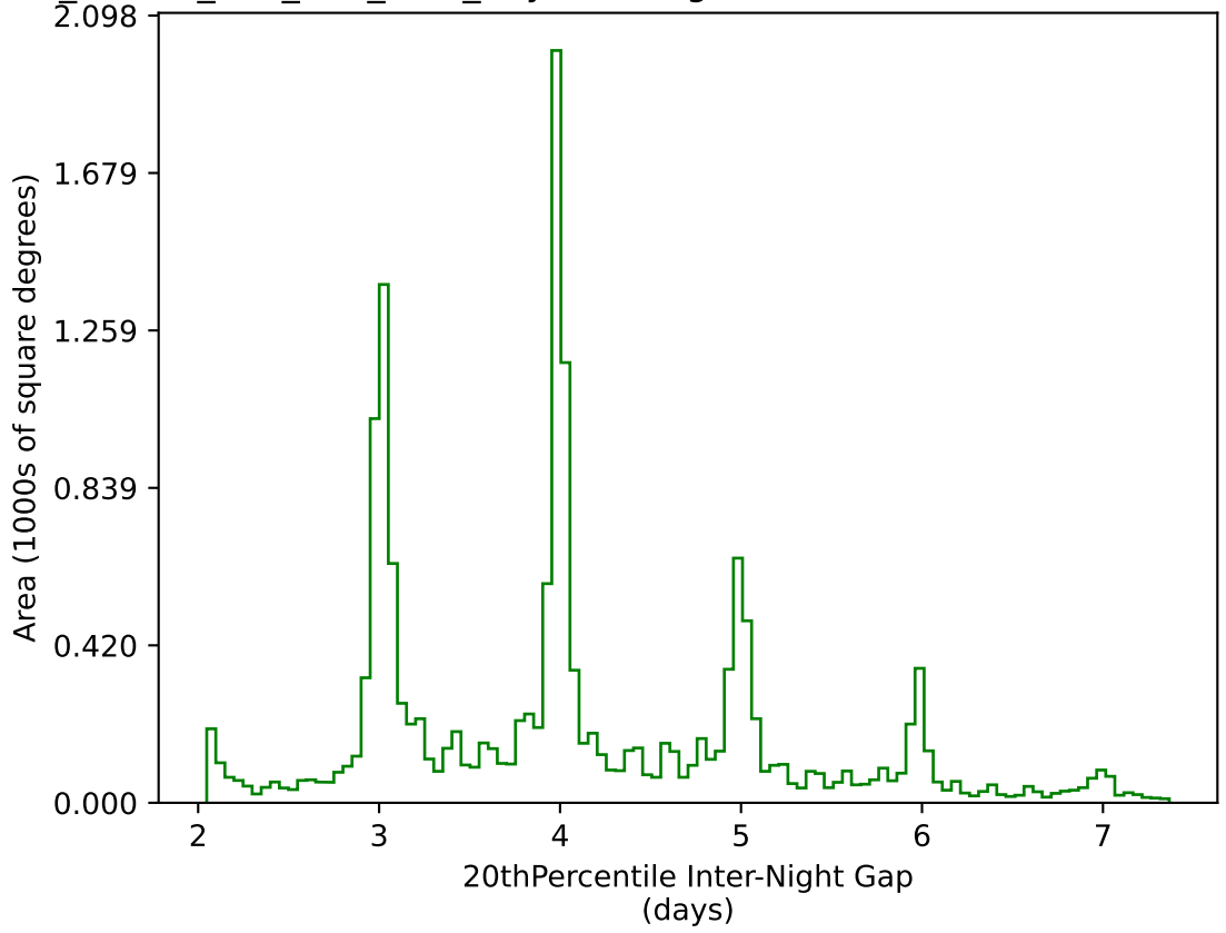
ddf_loaded_half_fl15_v3.4_10yrs WFD g band: 20thPercentile Inter-Night Gap
