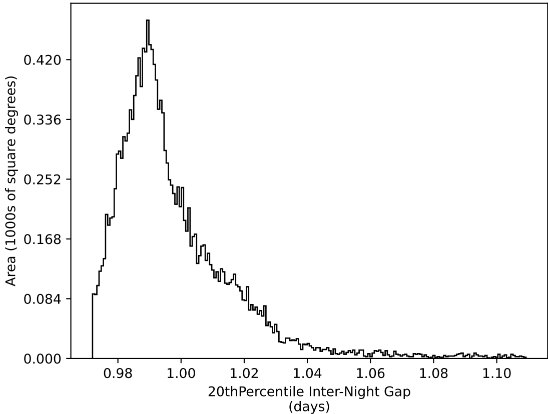
ddf_loaded_half_fl15_v3.4_10yrs WFD all bands: 20thPercentile Inter-Night Gap
