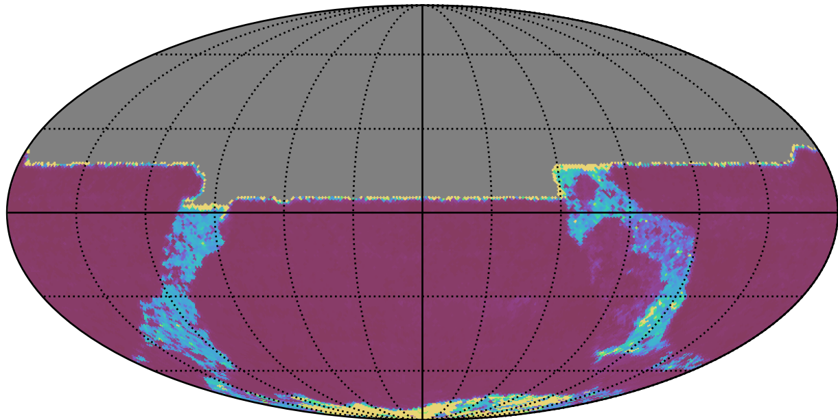
ddf_loaded_half_fl15_v3.4_10yrs All sky y band: 20thPercentile Inter-Night Gap
