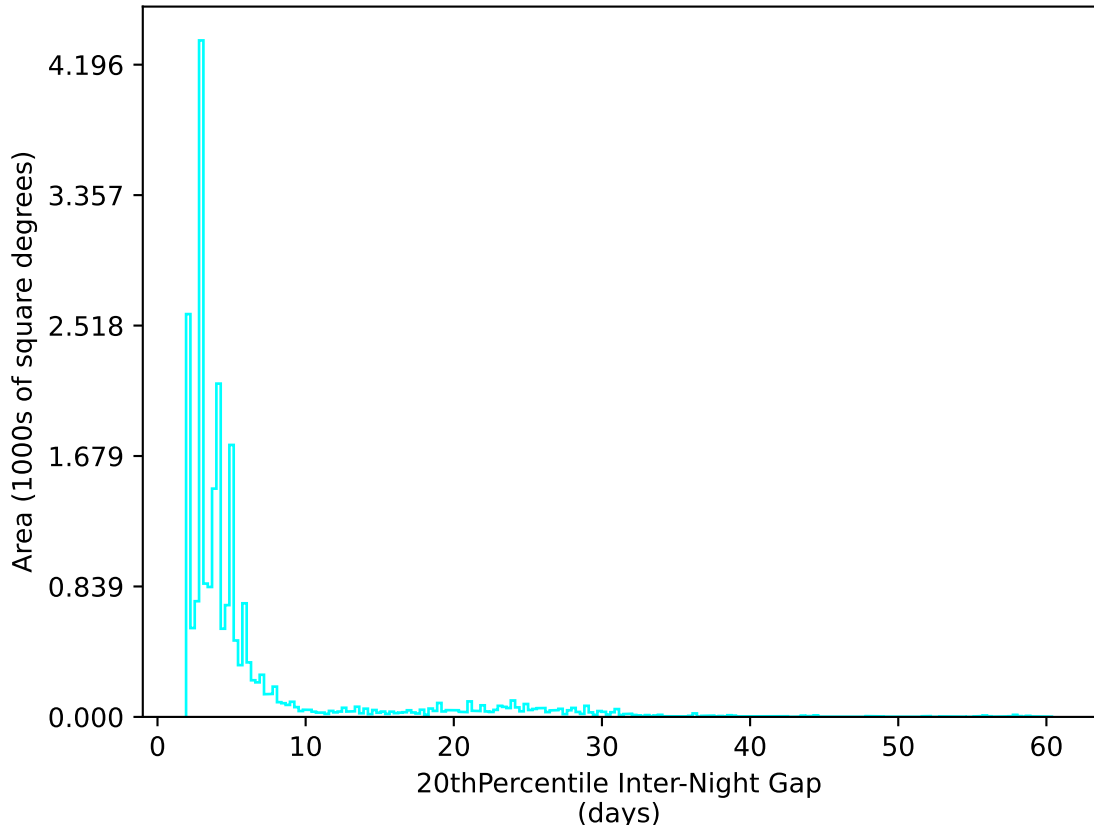
ddf_loaded_half_fl15_v3.4_10yrs All sky u band: 20thPercentile Inter-Night Gap
