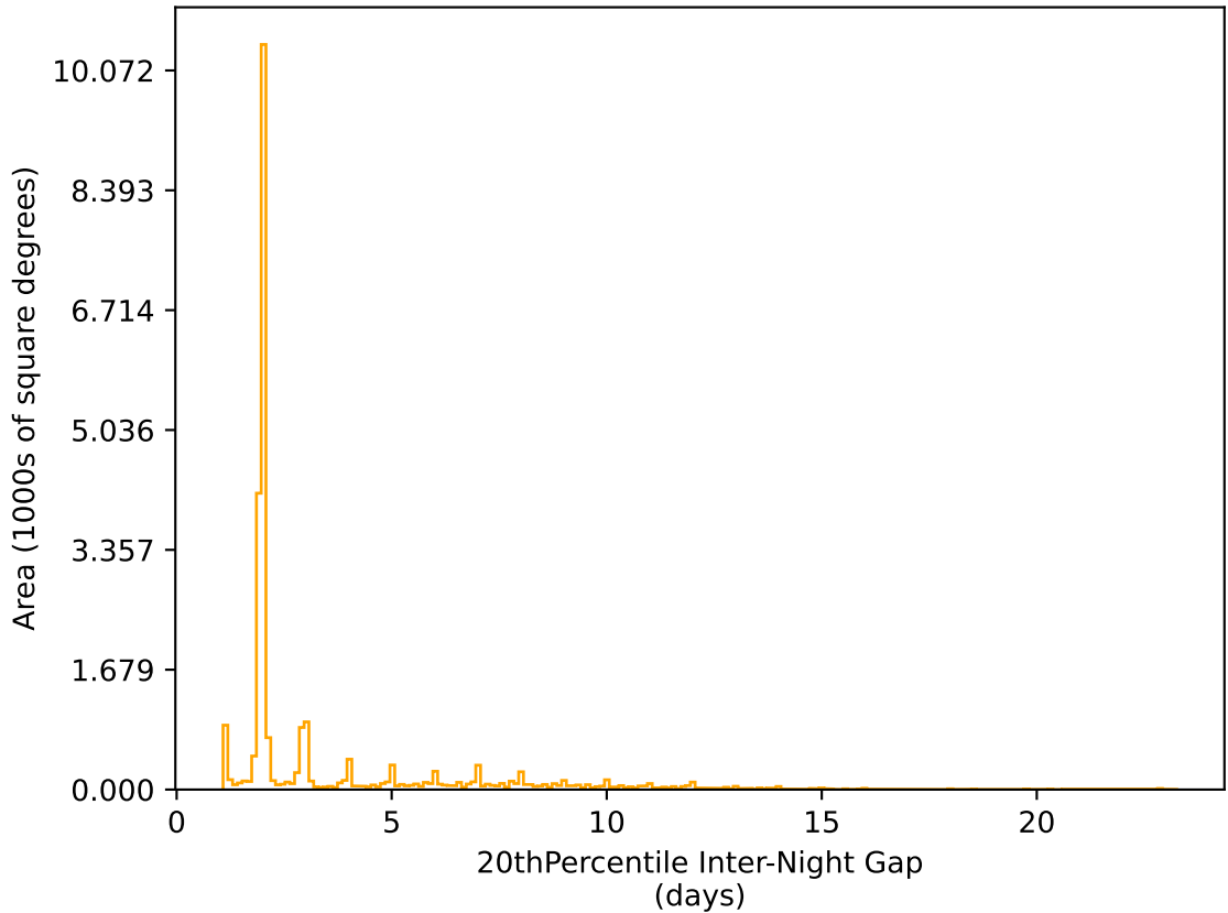
ddf_loaded_half_fl15_v3.4_10yrs All sky r band: 20thPercentile Inter-Night Gap
