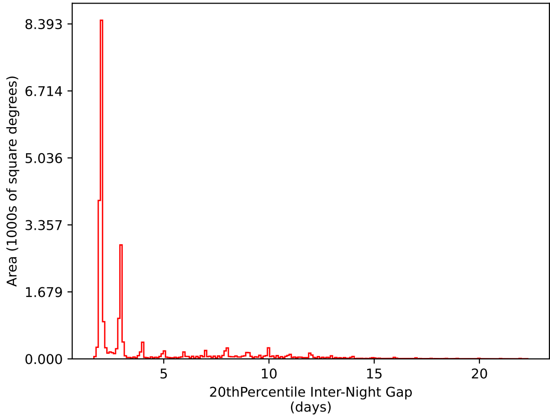
ddf_loaded_half_fl15_v3.4_10yrs All sky i band: 20thPercentile Inter-Night Gap
