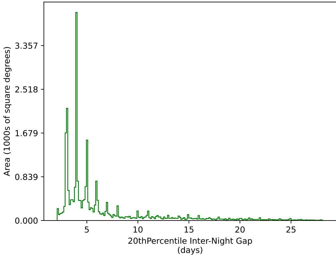
ddf_loaded_half_fl15_v3.4_10yrs All sky g band: 20thPercentile Inter-Night Gap
