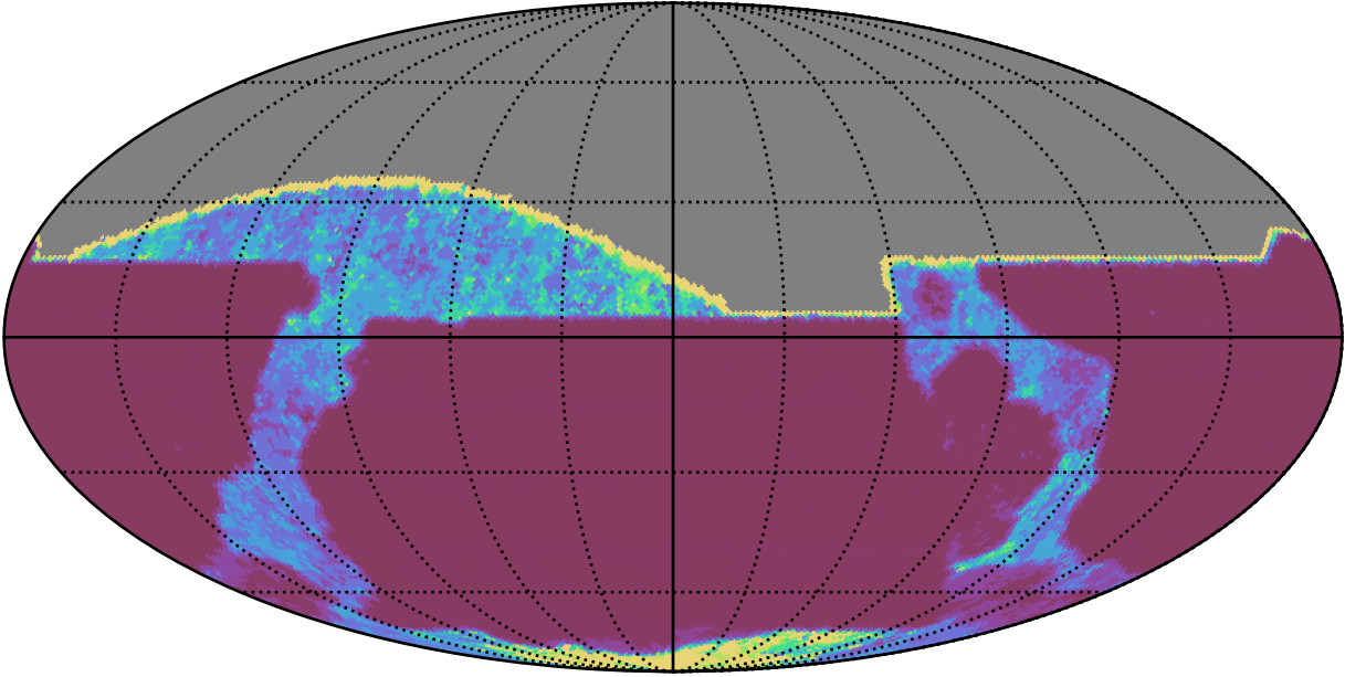
ddf_loaded_half_fl15_v3.4_10yrs All sky all bands: 20thPercentile Inter-Night Gap
