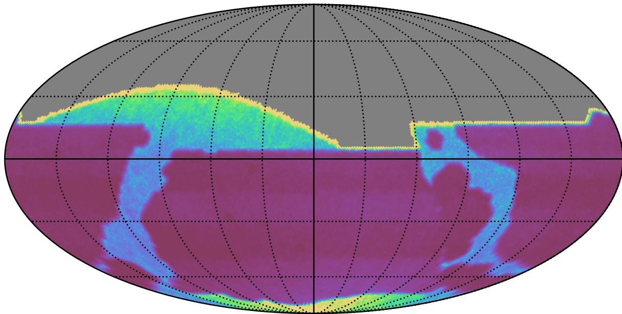
ddf_loaded_half_fl15_v3.4_10yrs : properMotion
