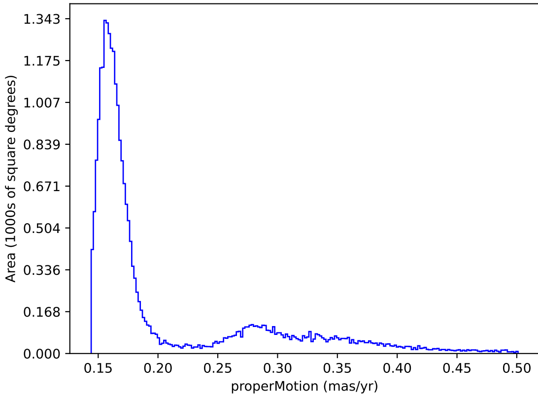
ddf_loaded_half_fl15_v3.4_10yrs : properMotion
