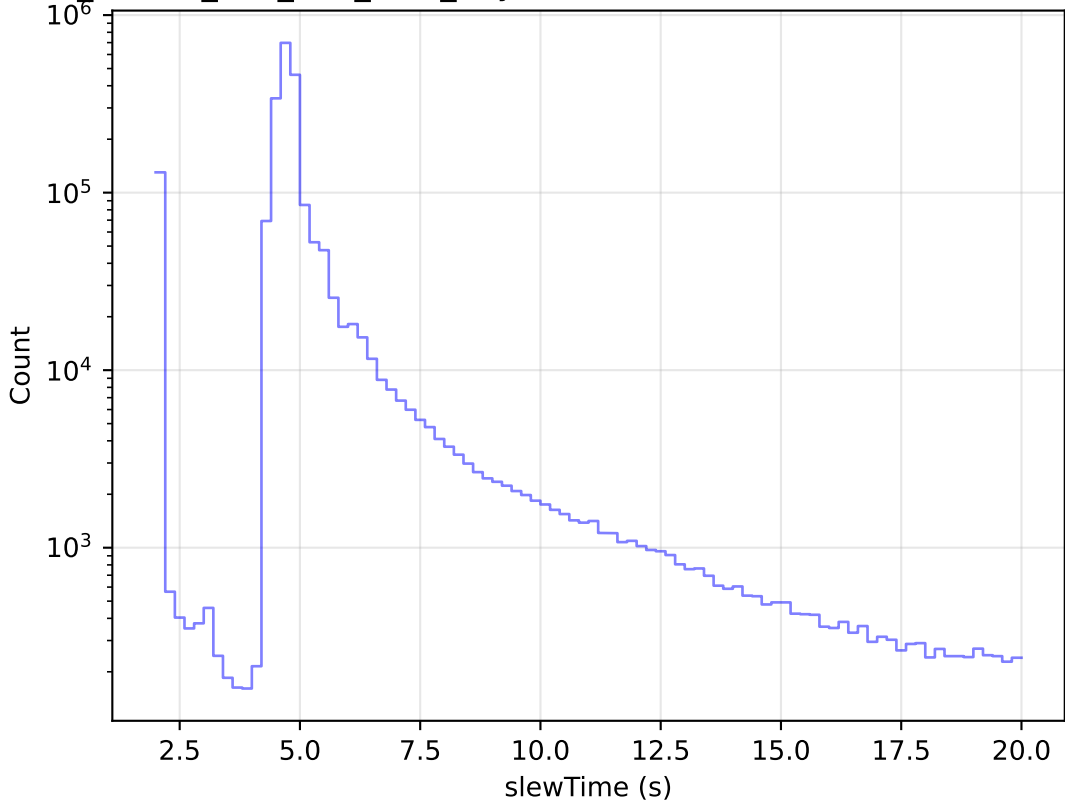
ddf_loaded_half_fl15_v3.4_10yrs All visits: Zoom Slew Time Histogram
