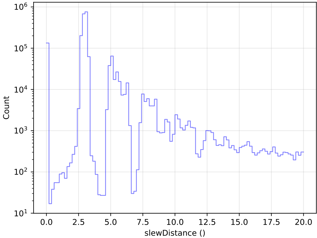
ddf_loaded_half_fl15_v3.4_10yrs All visits: Zoom Slew Distance Histogram
