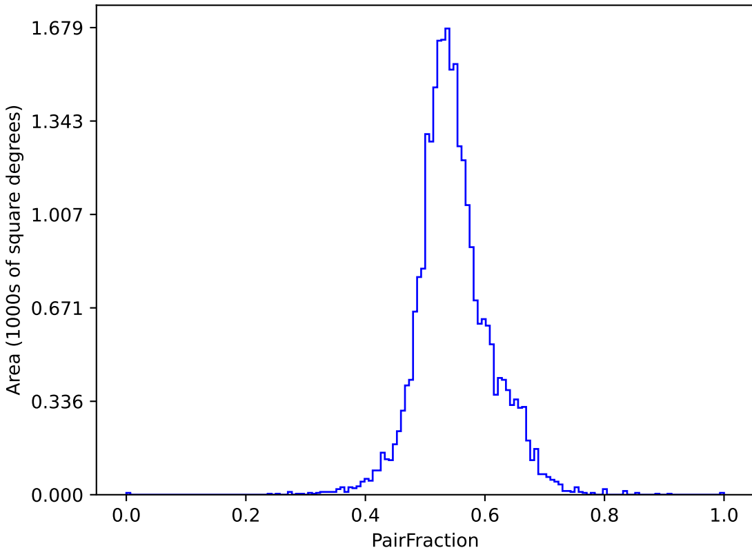
ddf_loaded_half_fl15_v3.4_10yrs (g or r or i): PairFraction
