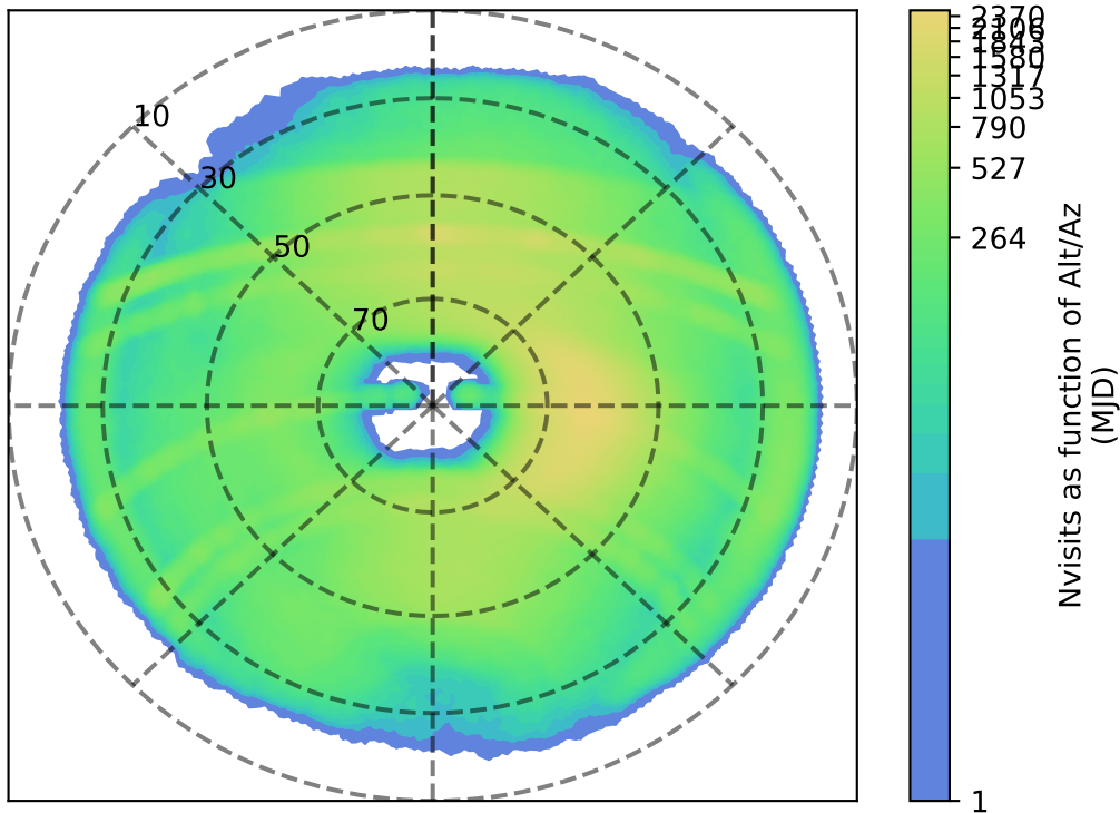
ddf_loaded_half_fl15_v3.4_10yrs i: Nvisits as function of Alt/Az
